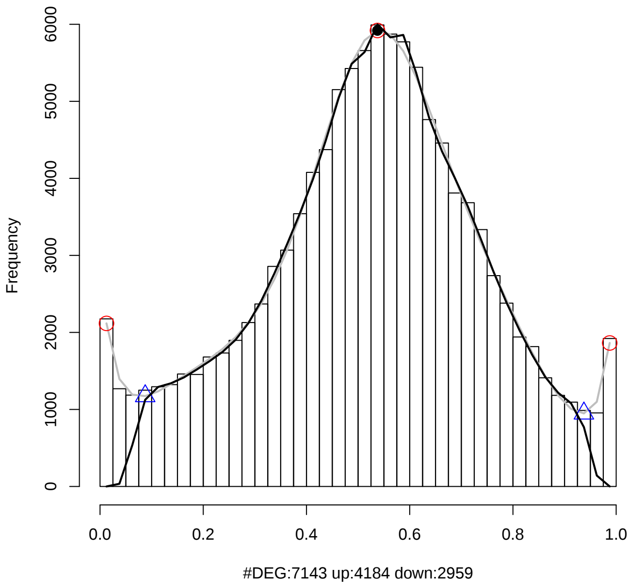
Histogram of P(\mu_{g2} - \mu_{g1} < 0) ; df=9
